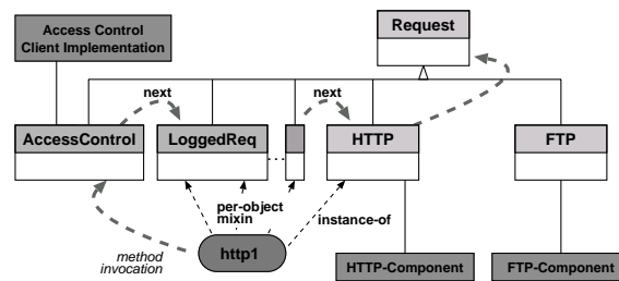
Figure 4. Request Logging/Access Control with Per-Object Mixins
