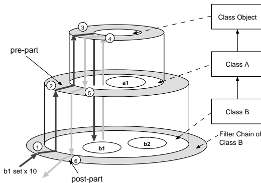
Figure 3: Filter Inheritance
