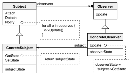
Figure 9: The Observer Pattern [10]
