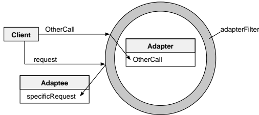
Figure 6: The Adapter Pattern Using Filters
