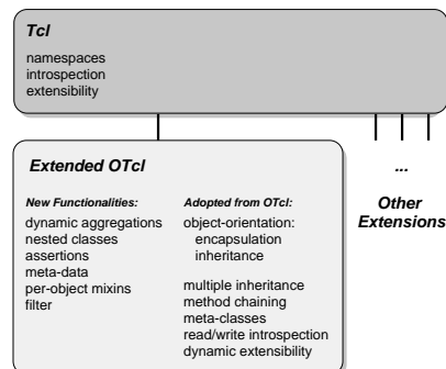
Figure 1: Language Extensions of XOTcl
