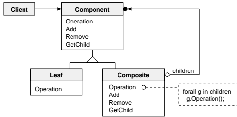
Figure 7: The Composite Pattern [10]
