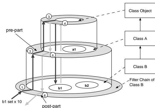
Figure 3: Filter Inheritance
