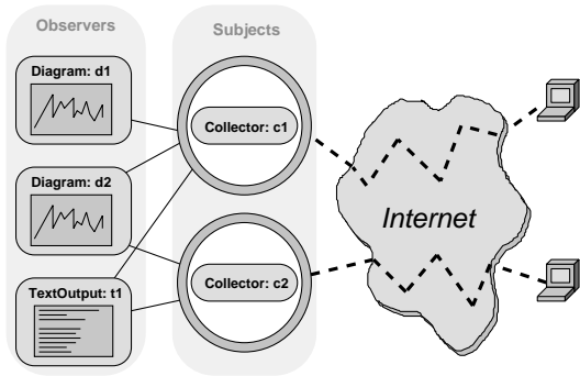
Figure 10: Observer Example
