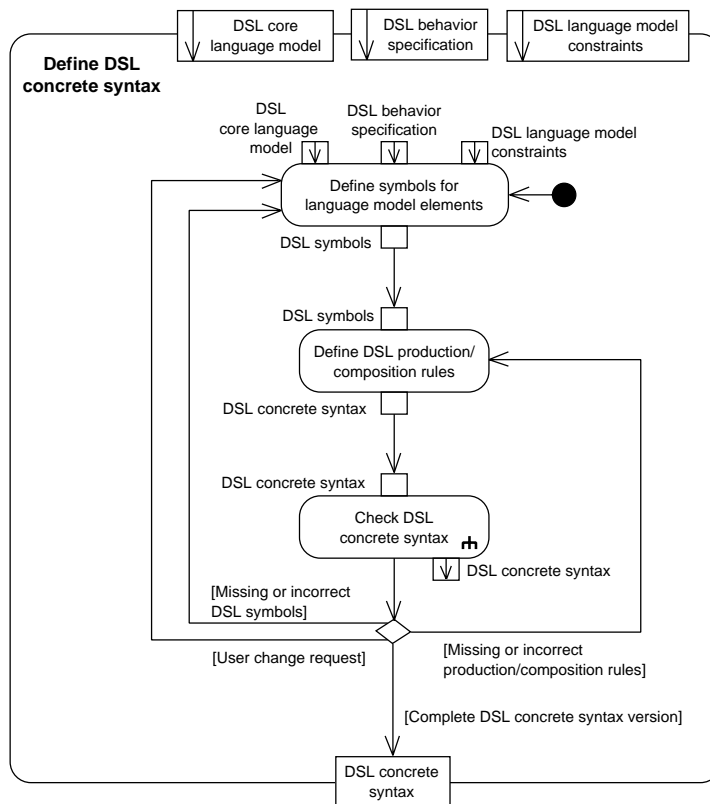
Figure 6. Subprocess: Define DSL Concrete Syntax
