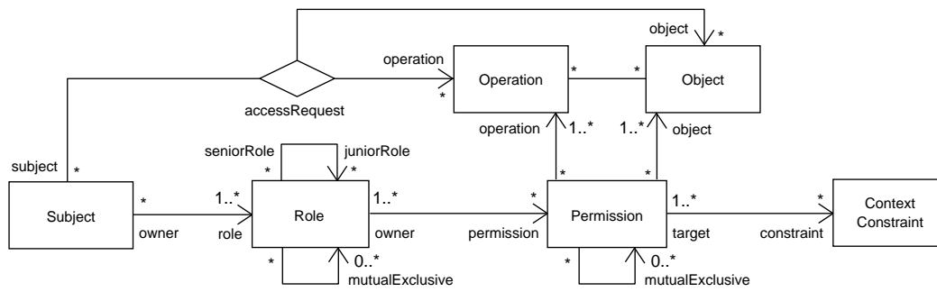
Figure 12. Core language model of the target domain: role-based access control
