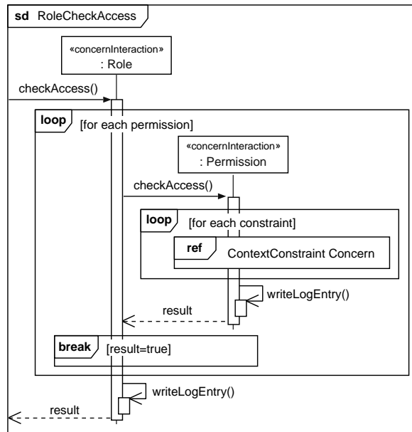
Figure 17. Interaction model for the Role concern [66]
