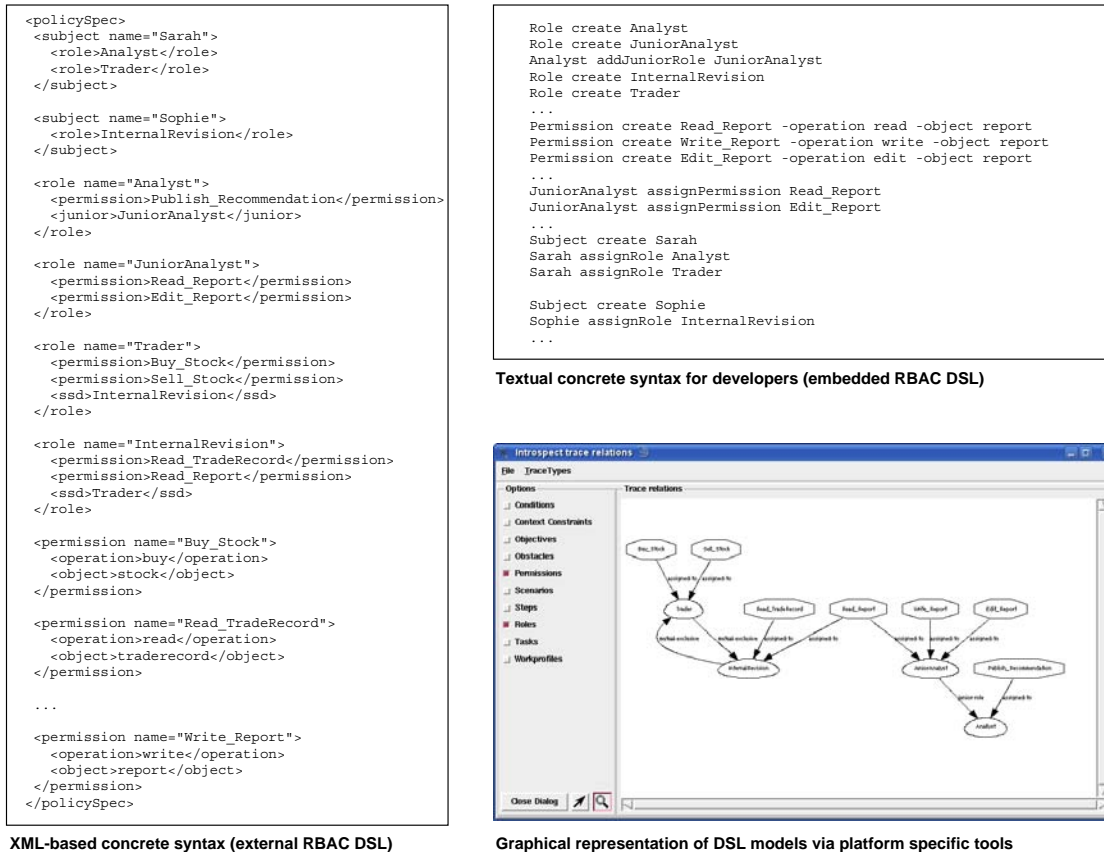
Figure 14. Concrete syntaxes of our RBAC DSL
