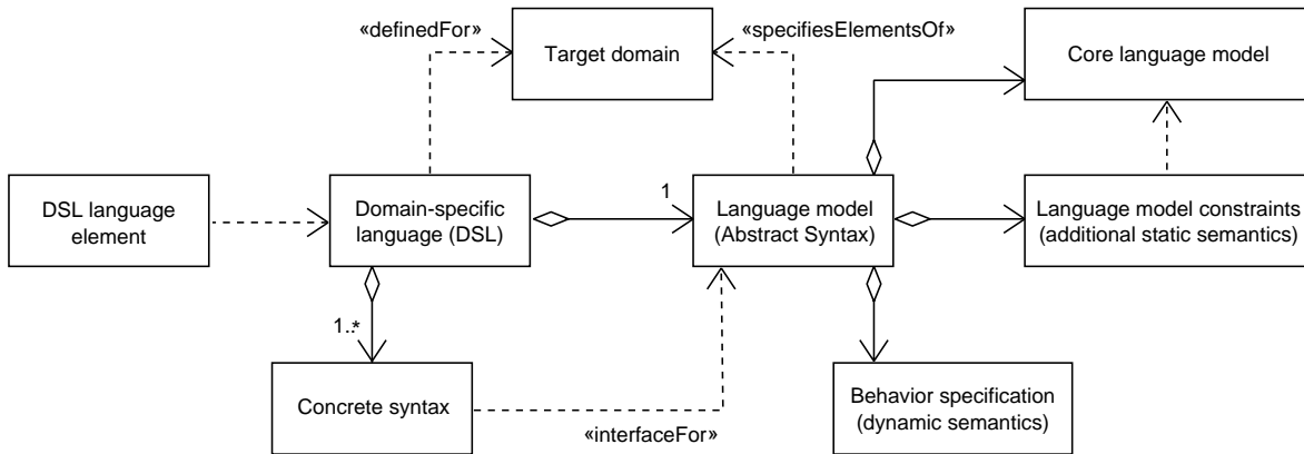
Figure 1. Domain-specific languages: Artifacts
