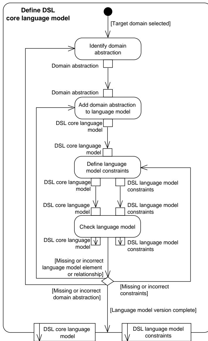
Figure 4. Subprocess: Define DSL Core Language Model
