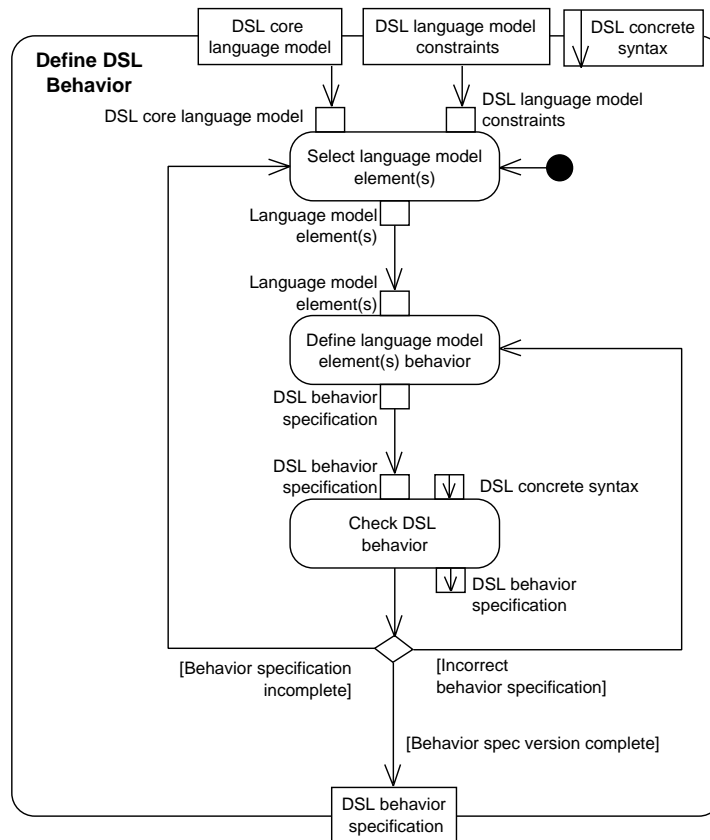
Figure 5. Subprocess: Define DSL Behavior
