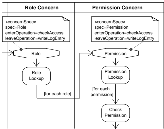
Figure 16. The Role and Permission Concerns with concernSpec stereotypes [66]
