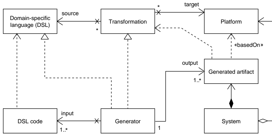
Figure 2. DSL transformations: Artifacts (loosely based on [61])
