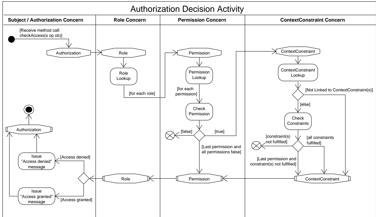
Figure 13. Control flow of the authorization concern [66]
