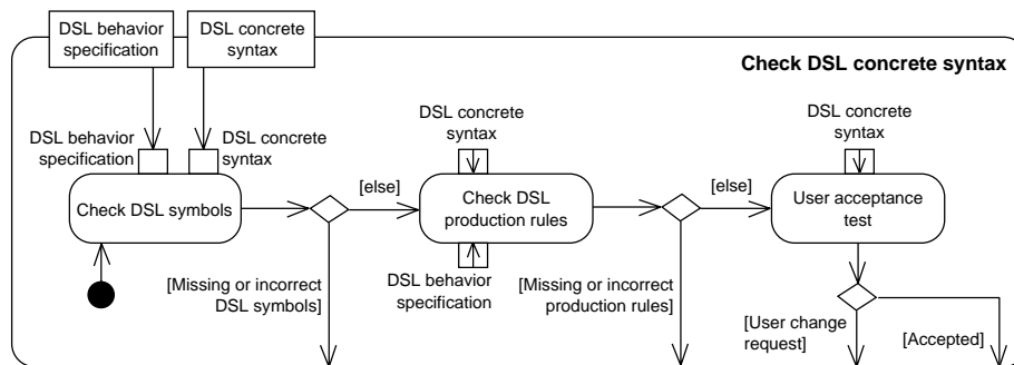
Figure 7. Checking concrete syntax artifacts
