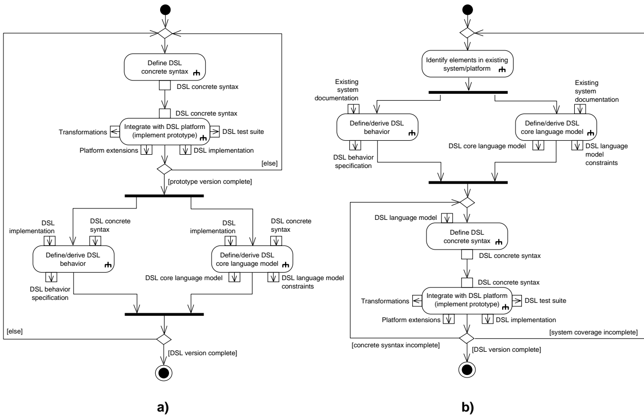
Figure 11. Examples of tailored process variants for DSL engineering
