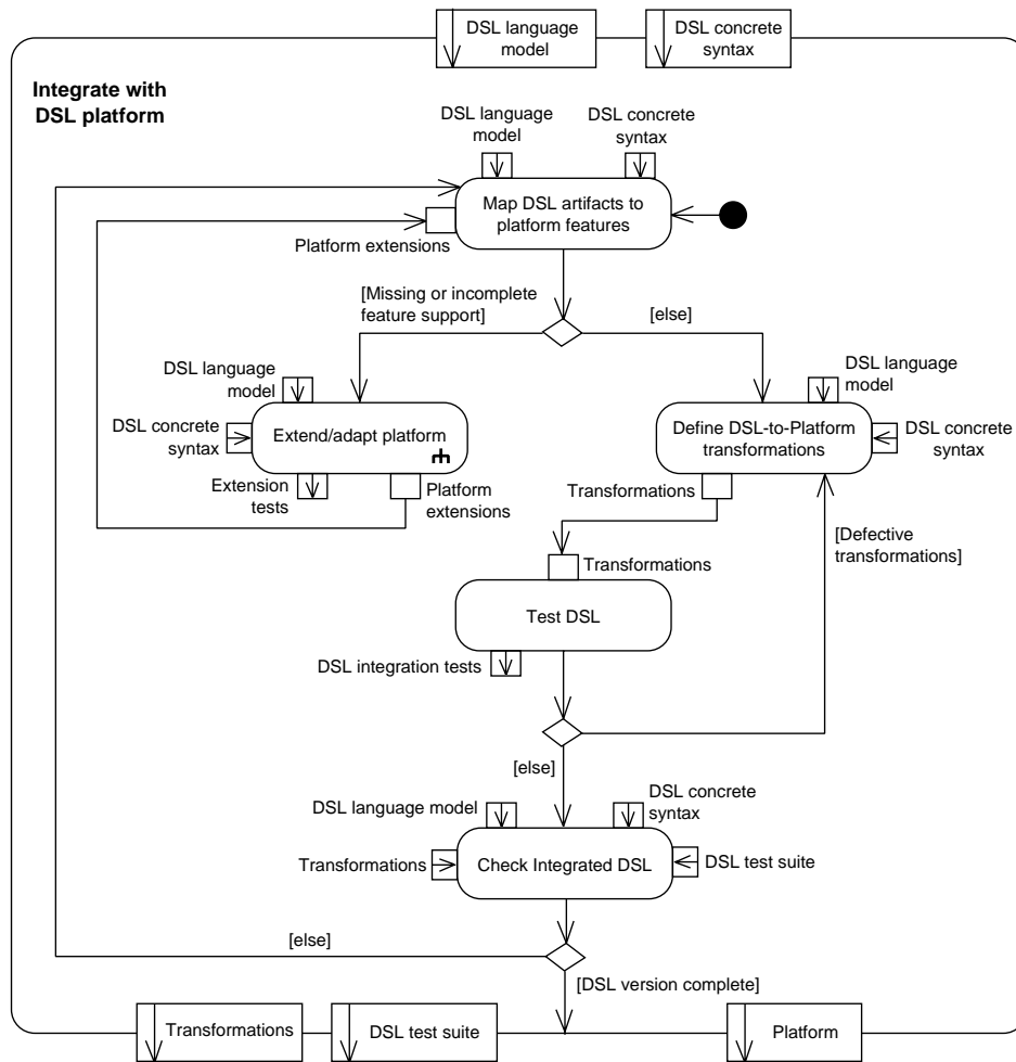
Figure 8. Subprocess: Integrate with DSL Platform
