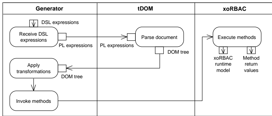
Figure 20. Transformation of DSL expressions: Activity model
