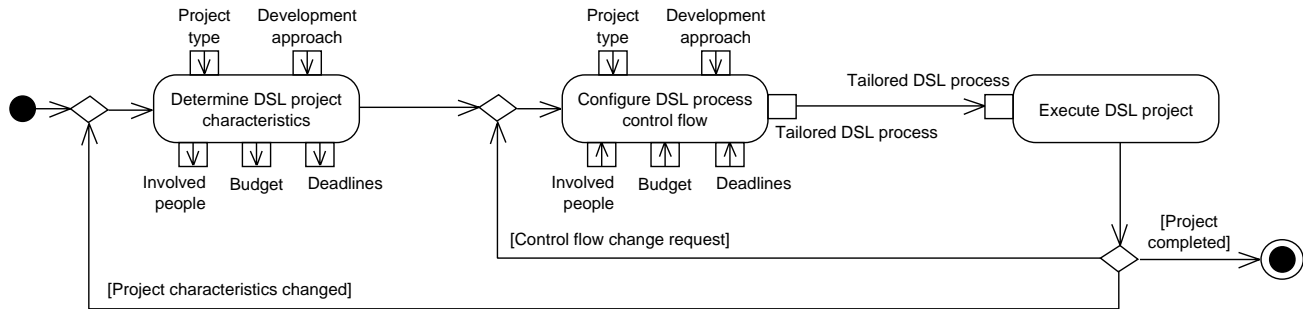
Figure 10. Project-specific tailoring of the DSL engineering process
