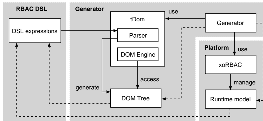
Figure 18. Transformation of DSL expressions: Structural overview
