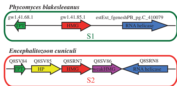
FIG. 1. —Gene arrangements in the MAT locus of Phycomyces blakesleeanus and in the corresponding gene cluster of Encephalitozoon cuniculi . In the sex-related region of P. blakesleeanus (S1), the gene encoding the sex-determining transcription factor (HMG) is flanked by two genes coding for a sugar transporter (TPT) and an RNA helicase, respectively. The corresponding cluster in E. cuniculi (S2) contains also genes for a TPT, an HMG-type transcription factor, and an RNA helicase. The two additional genes in S2 encode a hypothetical protein (HP) and a protein with a weak similarity to a HMG domain protein.
