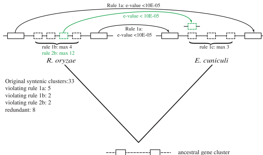
FIG. 4. —Reanalysis of the proposed shared syntenic gene clusters between Rhizopus oryzae and Encephalitozoon cuniculi . Two decision rules were used to assign shared synteny (c.f. fig. S5 in Lee et al. 2008). Rule 1 requires that (1a) two R. oryzae genes have a Blast hit with an e-value < 10 \times 10^{-5} in E. cuniculi , (1b) the two R. oryzae genes must be separated by no more than four genes, and (1c) the corresponding E. cuniculi genes must be separated by no more than three genes. Rule 2 extends rule 1 if one of the intervening R. oryzae genes also has a Blast hit (e-value < 10 \times 10^{-5} ) in E. cuniculi . In this case, the R. oryzae genes must be separated by no more than 12 genes (2b). Please note that in the original publication, the decision rules were described for a search in the opposite direction, that is, with the E. cuniculi proteins as query. However, the data presented in table S1 of Lee et al. 2008 (c.f. also supplementary table 2, Supplementary Material online) are not compatible with this direction of the search. Hence, we adjusted the decision rules to fit the data.
