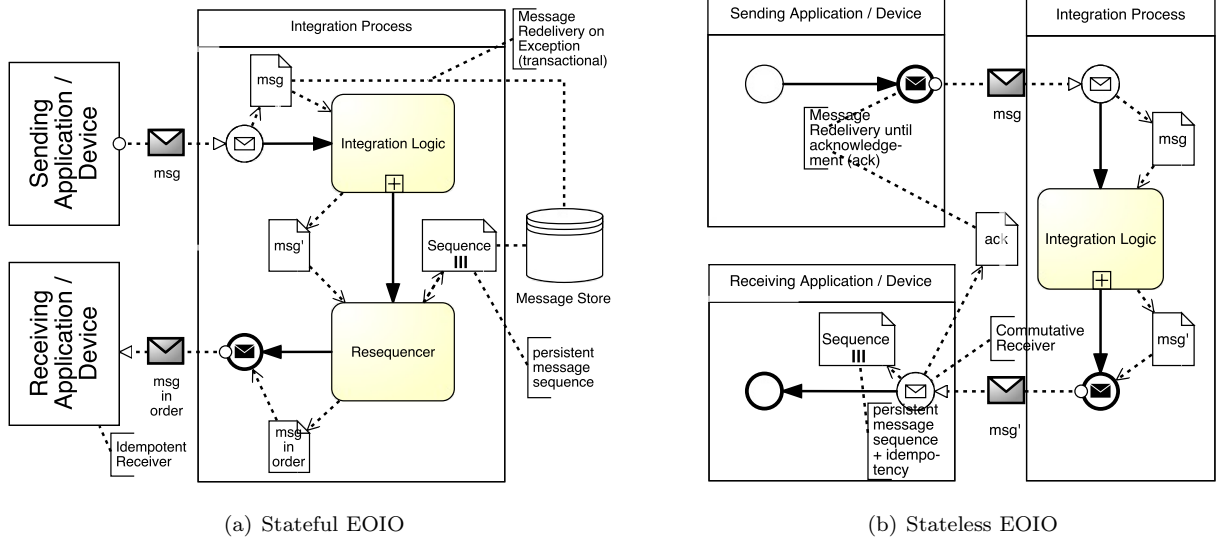
Figure 6: Conversational approach for Exactly Once in Order (EOIO).
