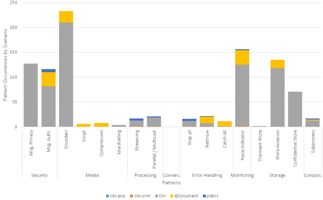
Figure 8: New capability categorization.
