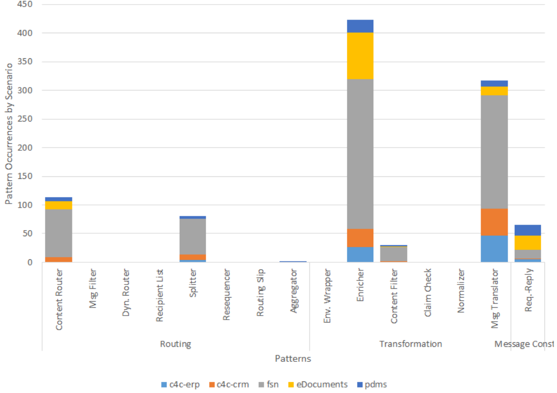
Figure 7: Scenarios using original EIP
