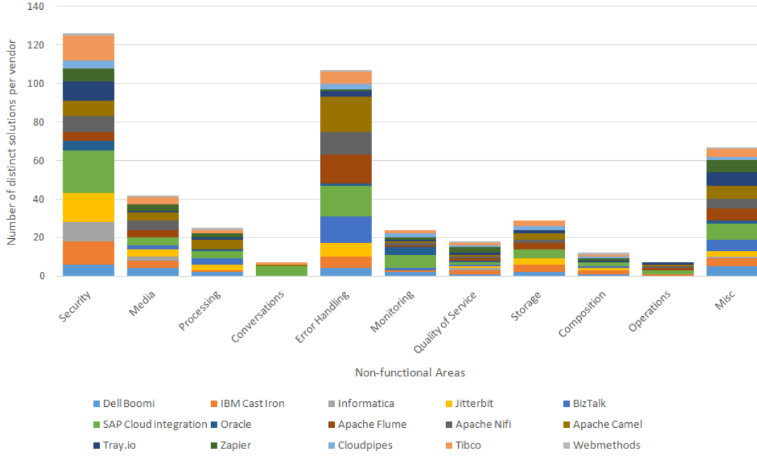
Figure 5: Solutions for NFA not covered by the EIP by system vendor.
