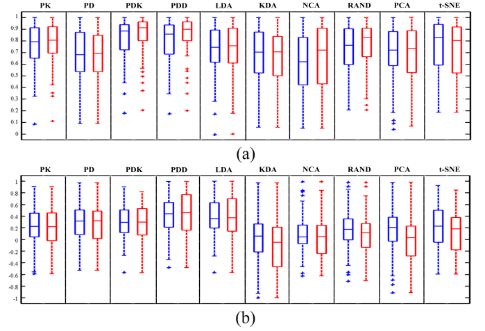
Fig. 8. These boxplots summarize the values of GONG (a) and SC (b) for the ten different DR methods, where the blue boxplots show the score distributions over all 93 datasets and red boxplots describe the score of the 53 real datasets only .
