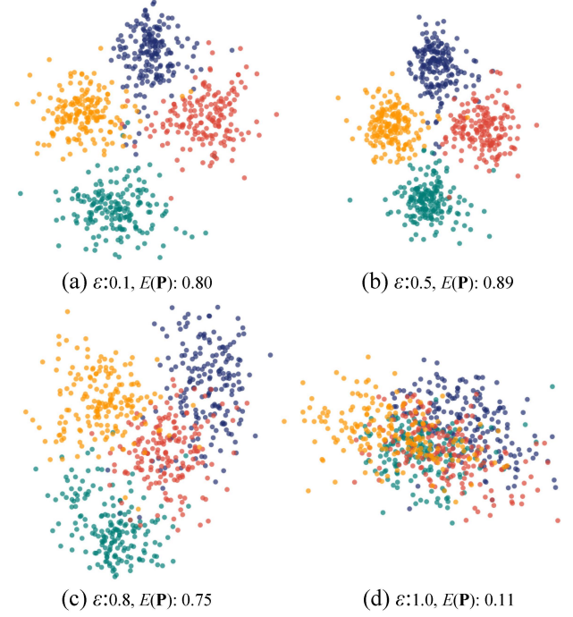
Fig. 5. These four results (a-d) are produced using different values of \epsilon : 0.1, 0.5, 0.8, and 1.0. Their final energies E(\mathbf{P}) are 0.80, 0.89, 0.75 and 0.11, respectively, while the running time are 9.94s, 2.40s, 0.81s and 0.04s, respectively.
