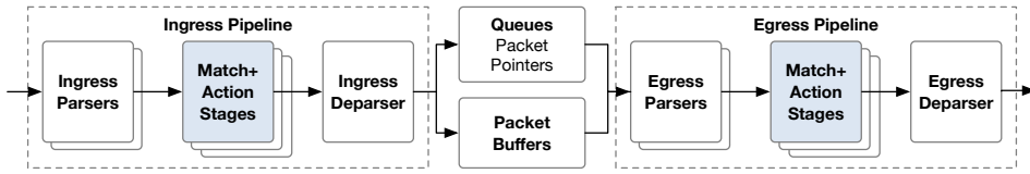
Fig. 3. The architecture of an RMT-like switching ASIC
