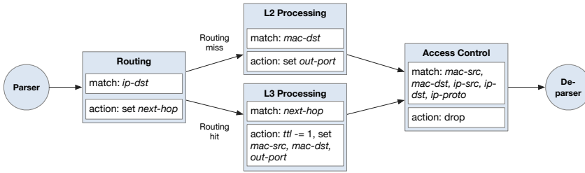
Fig. 4. Simplified match-action table dependency graph for a basic router (inspired by Fig. 3 in [22]).
