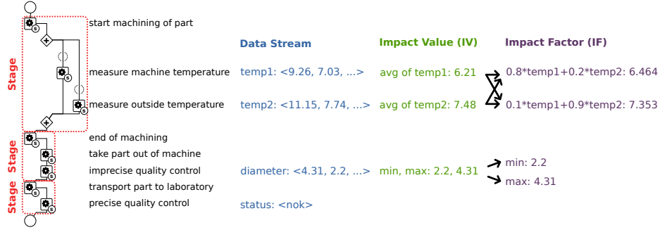
Fig. 4: Running Example Process
