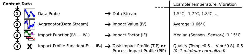
Fig. 3: Impact Profiles and Related Concepts
