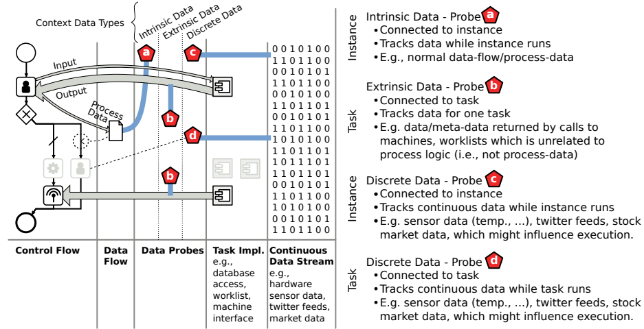
Fig. 2: Types of Data in the Process Context
