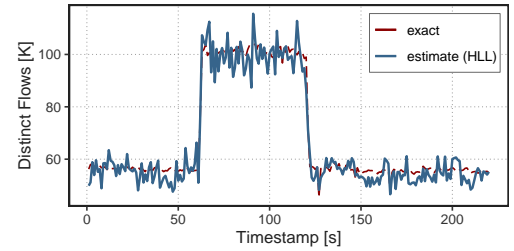
Figure 8. HyperLogLog flow count estimate and ground truth during a flooding attack.
