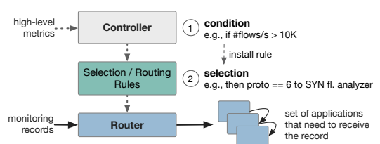
Figure 3. Router overview
