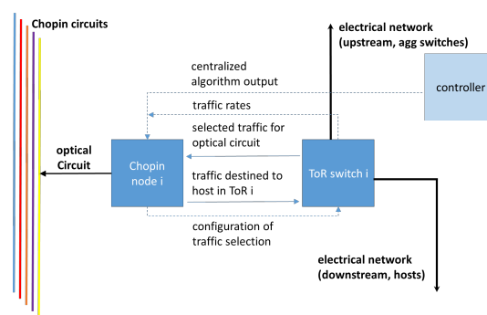
■ Figure 2 Chopin's design.
