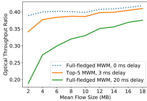
Figure 4 Comparison between a centralized scheduler which operates every 3 ms and computes the MWM of the top-5 live flows, to a centralized scheduler which operates every 20 ms and computes full-fledged MWM. For brevity only pFabric results are shown.
