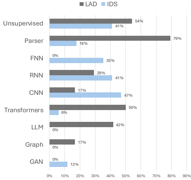
Figure 5: Distribution of primary keywords in the literature related to publications on Log Anomaly Detection (LAD) and Intrusion Detection Systems (IDS).
