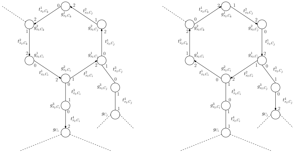
Figure 1: An excerpt of the game graph for variable x_\ell which occurs in clauses C_i and C_k positively and in C_j negatively. In the left image the outcomes of the games for x_\ell = \text{true} are visualised, in the right image we have x_\ell = \text{false} . The edges are directed towards the game that was won by the corresponding team; the numbers close to the game vertices show how many points the associated two-game teams win in this game.
