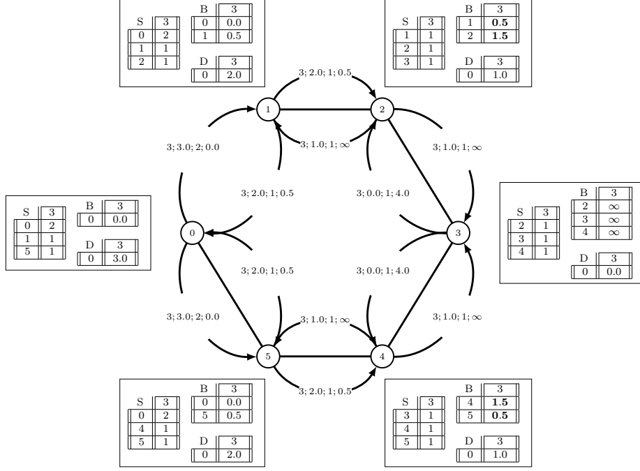
Figure 3: The state of Algorithm 2 executed on a cycle of 6 nodes, at the end of the sixth send/receive phase of the algorithm.
