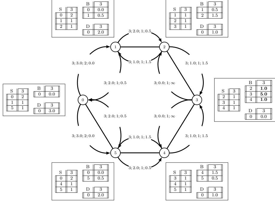
Figure 4: The state of Algorithm 2 executed on a cycle of 6 nodes, at the end of the seventh and last send/receive phase of the algorithm.
