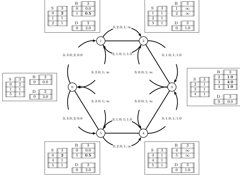
Figure 2: The state of Algorithm 2 executed on a cycle of 6 nodes, at the end of the fifth send/receive phase of the algorithm.
