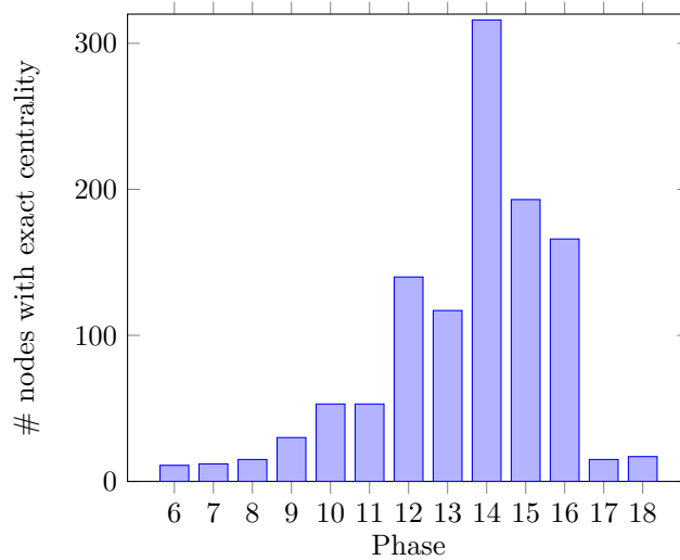
Figure 9: The number of nodes whose C value converges to the exact centrality value as a function of the phase, in the case of the autonomous system network.
