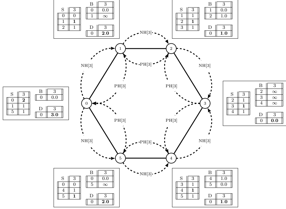
Figure 1: The state of Algorithm 2 executed on a cycle of 6 nodes, at the end of the fourth send/receive phase of the algorithm.
