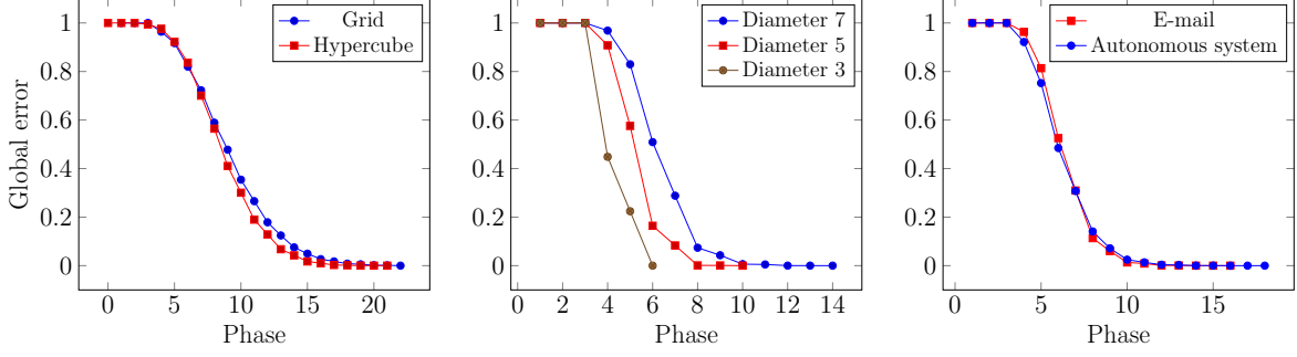
Figure 5: The (mean) global error as a function of time in (left) a 7 \times 6 grid and a hypercube of dimension 11 (where, hence, diameter is 11), (center) Erdős-Renyi graphs with 500 nodes and different diameters (20 samples for each diameter), and (right) an e-mail network with 1133 nodes and in an autonomous system network with 3011 nodes.
