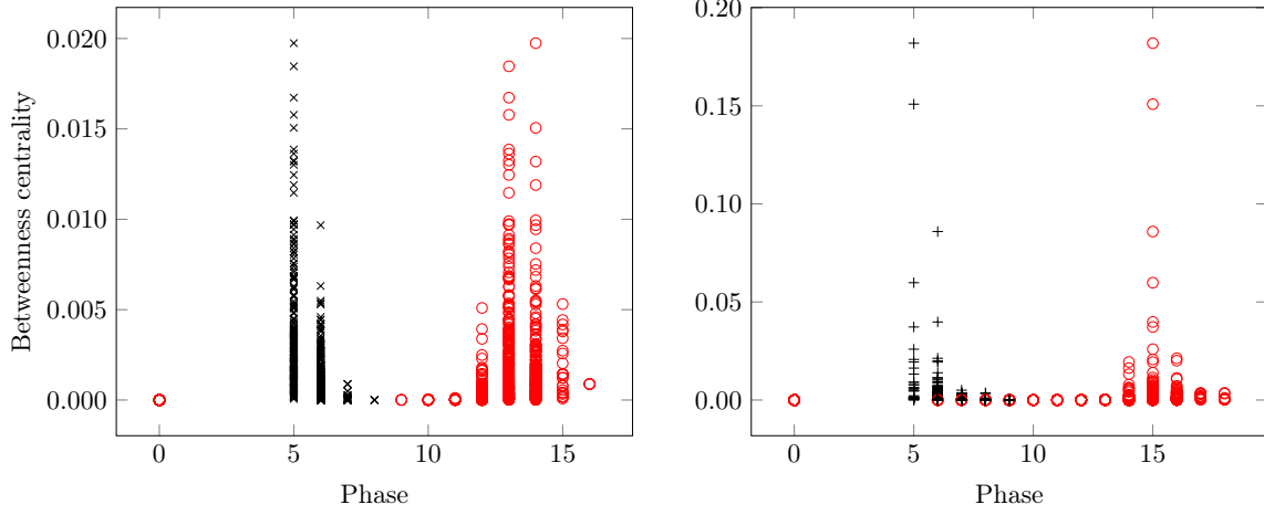
Figure 8: T_D and T_C for all the nodes of the e-mail network (left) and of the autonomous system network (right).
