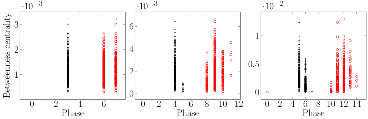
Figure 7: T_D and T_C for all the nodes of three Erdős-Rényi graphs with diameter 3, 5, and 7, respectively.
