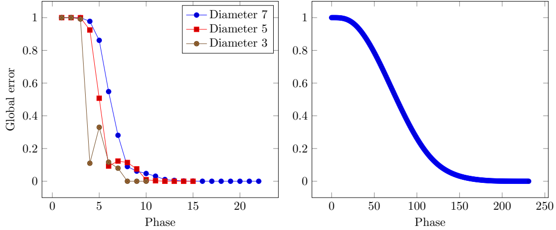
Figure 6: The (mean) global error as a function of time in randomly weighted Erdős-Rényi with 500 nodes (20 samples per diameter, where the noted diameter is the one of the underlying, unweighted graphs), and in a road network with 3353 vertices.
