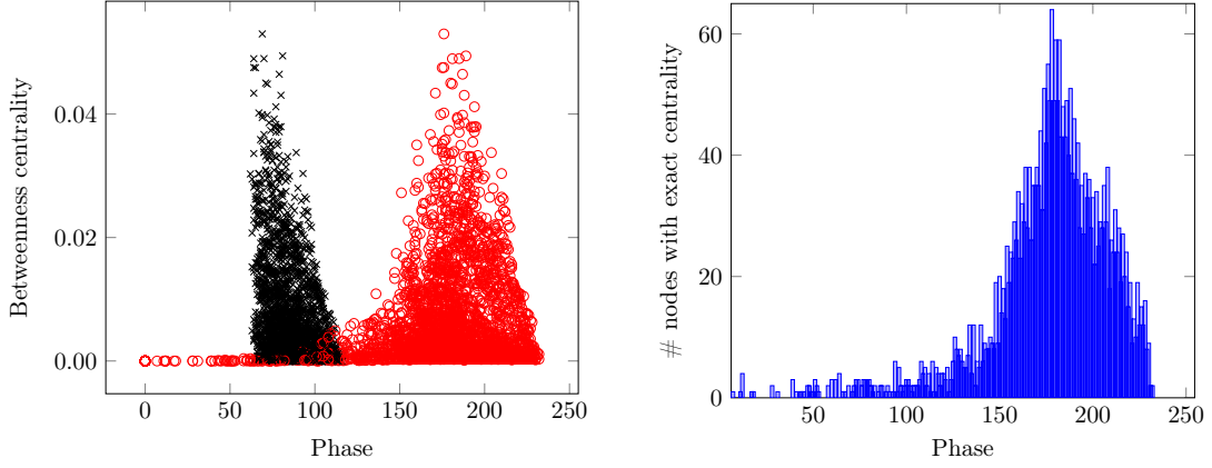
Figure 10: T_D and T_C for all the nodes (left) and number of nodes whose C value converges to the exact centrality value as a function of time (right), in the case of the road network.
